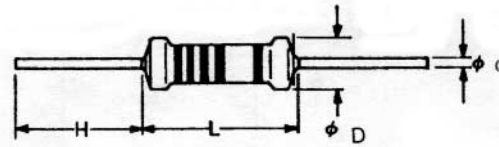
DIMENSIONS: (mm)
