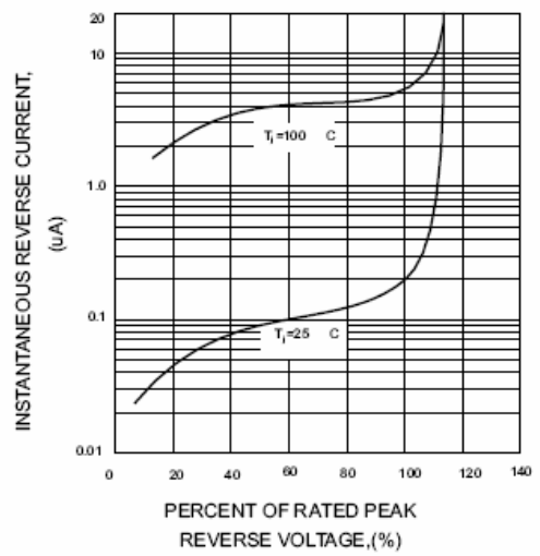
FIG.4-TYPICAL REVERSE CHARACTERISTICS
