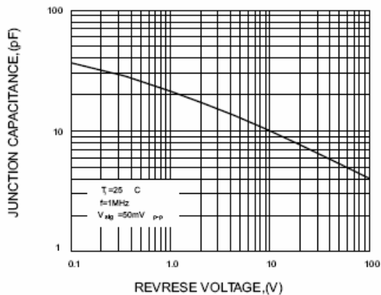
FIG.5-TYPICAL JUNCTION CAPACITANCE
