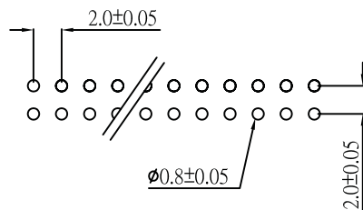
RECOMMENDED P.C.B BOARD HOLE LAYOUT
