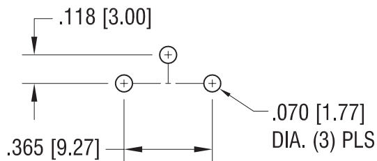
MOUNTING DETAIL
