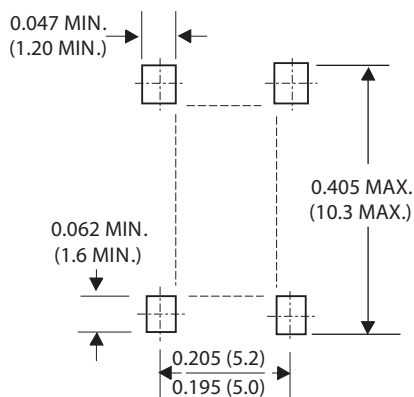
Fig. 5 Mounting Pad Layout
