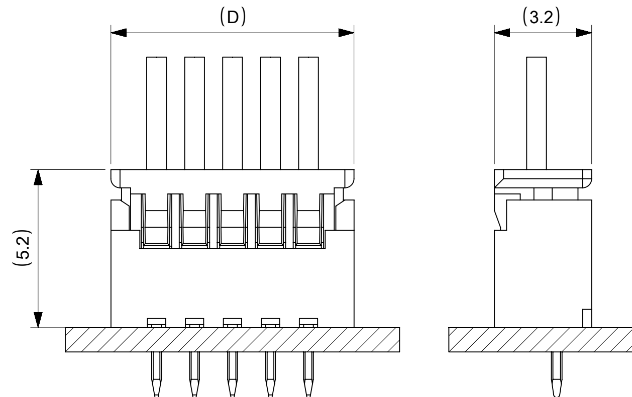
1 嵌合図 MATED CONNECTOR
