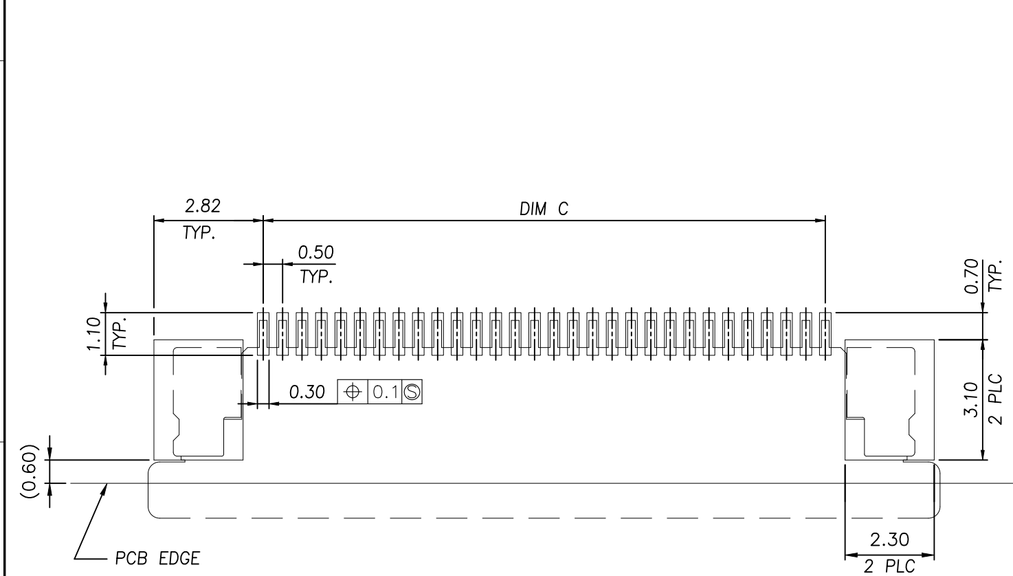
RECOMMENDED PCB DIMENSIONS DIAGRAM TOLERANCE: ±0.05
