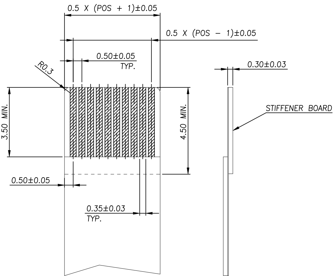
RECOMMENDED FPC DIMENSIONS DIAGRAM
