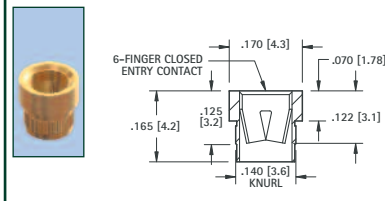
.084 (2.13) - .102 (2.6) PIN - PRESS-FIT
