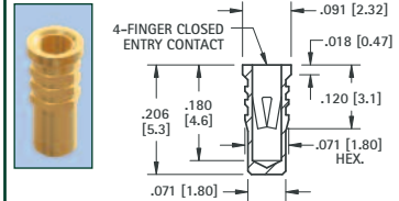
.032 (.81) - .046 (1.17) PIN - PRESS-FIT
