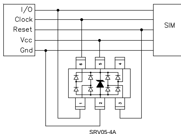
Figure 6 - SIM Port
