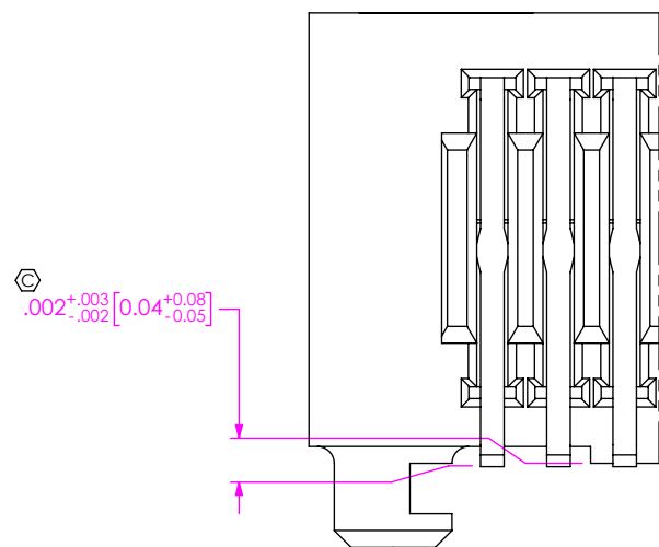
DETAIL 'H' SCALE 8 : 1
