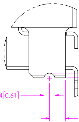
DETAIL 'F' SCALE 8 : 1
