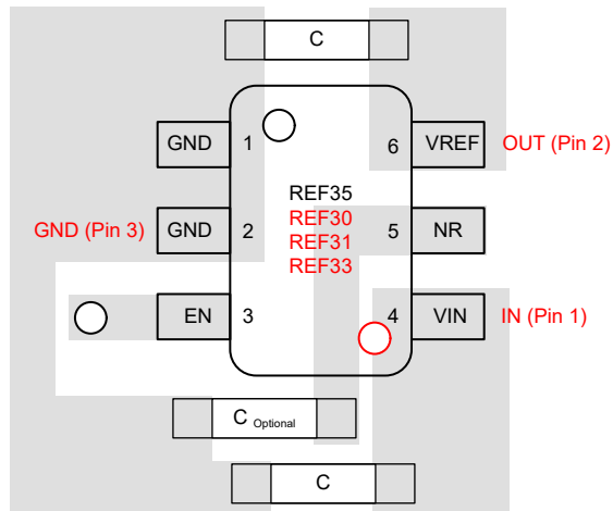
Figure 9-5. Pin Compatibility With REF30xx, REF31xx and REF33xx
