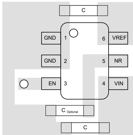
Figure 9-4. Layout Example - DBV package
