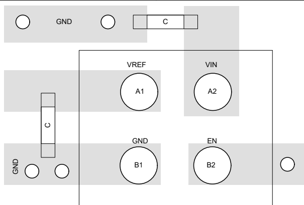
Figure 9-6. Layout Example - YBH package
