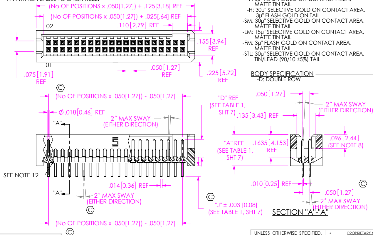
FIG 1 THROUGH HOLE -01, -03, -11, -13, -21, -23, -31
